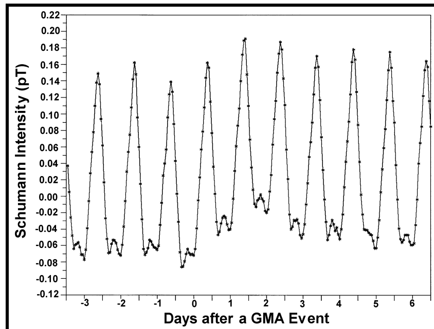
Figure 6: Superimposed epoch analysis of the impact of a Geomagnetic event, as defined by the Kp Index, for the mean anomaly in the Schumann Resonance 0-20 Hz intensity for 69 events in 1997 to 1999. GMA events occurred on day zero.
