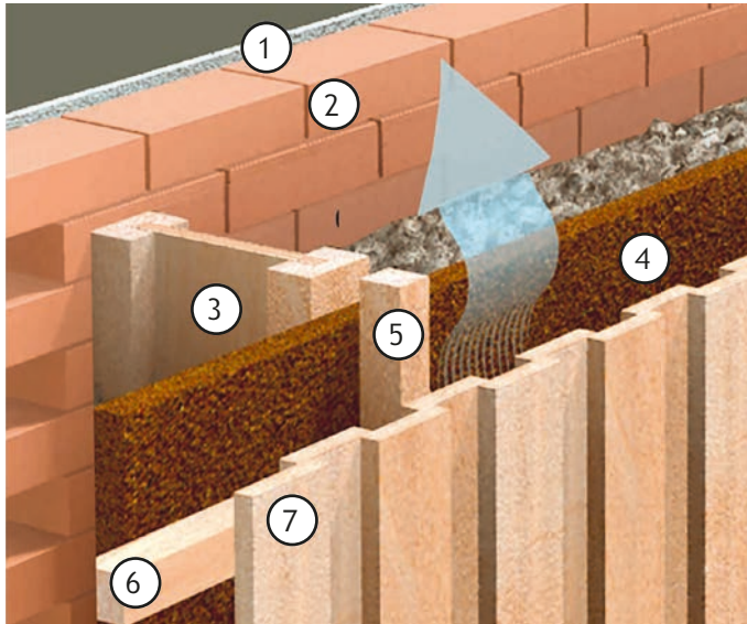
Hinterlüftete Fassade (FH Salzburg, Smart Building)
